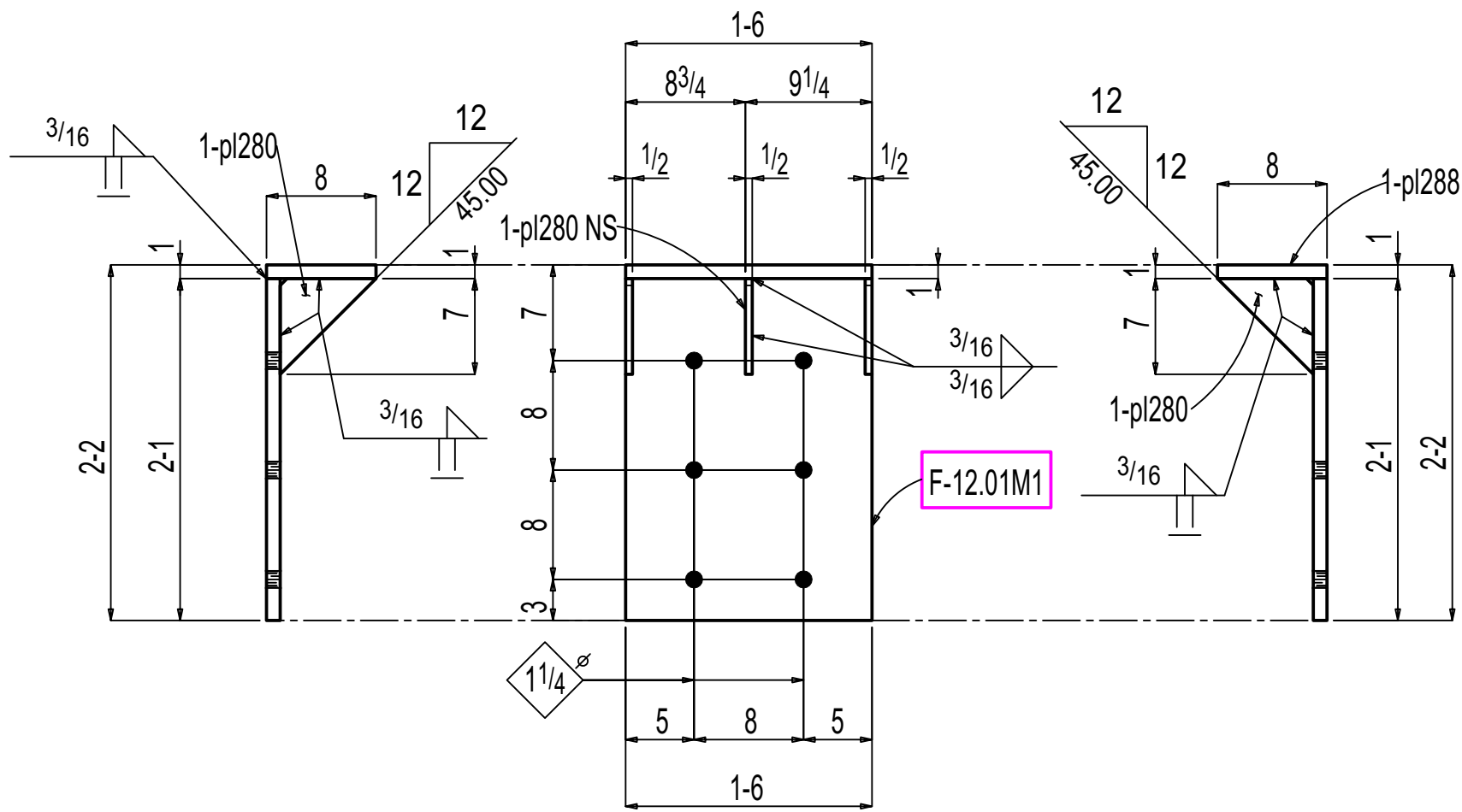
ONE PLATE F-12.01M1
