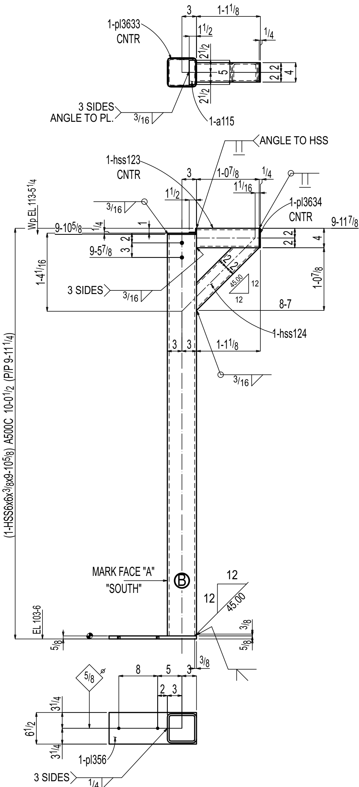
ONE COLUMN F-12.02C2
