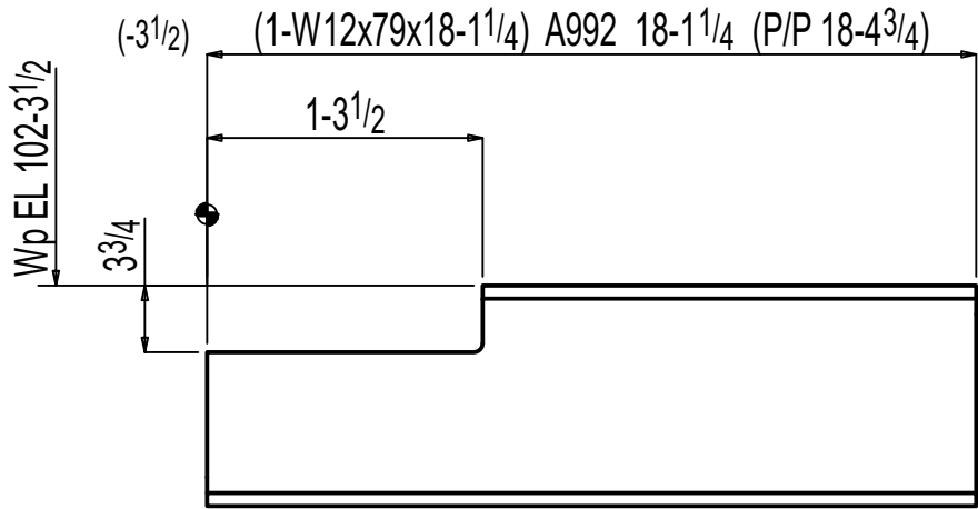
ONE BEAM F-12.02B1
