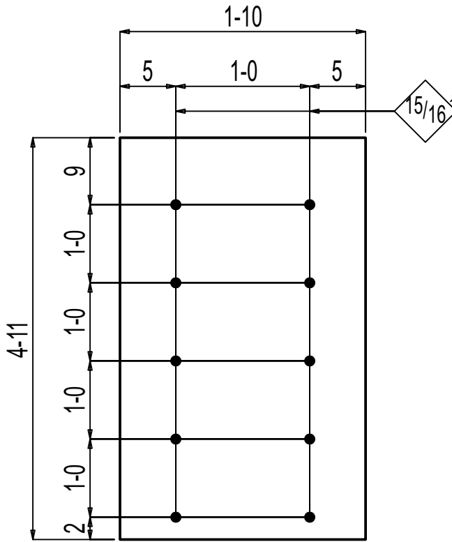
ONE EMBED PLATE F-12.01EP1
