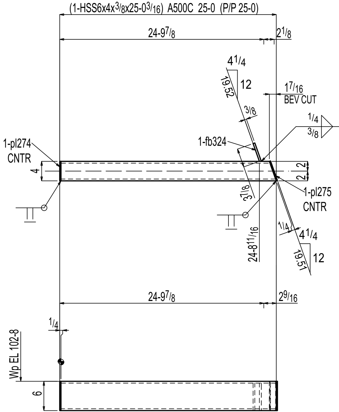
ONE BEAM F-12.02B4
