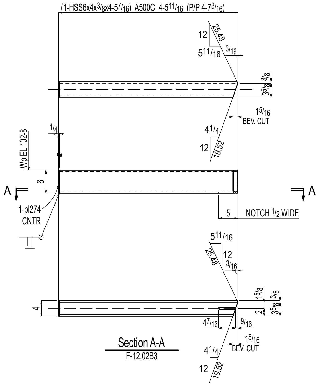
ONE BEAM F-12.02B3
