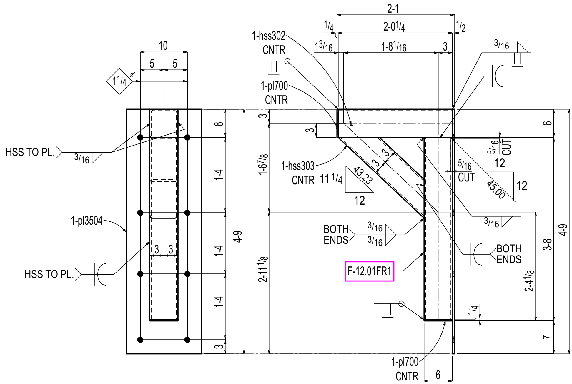
ONE FRAME F-12.01FR1
