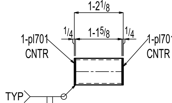
ONE HSS F-12.01M3
