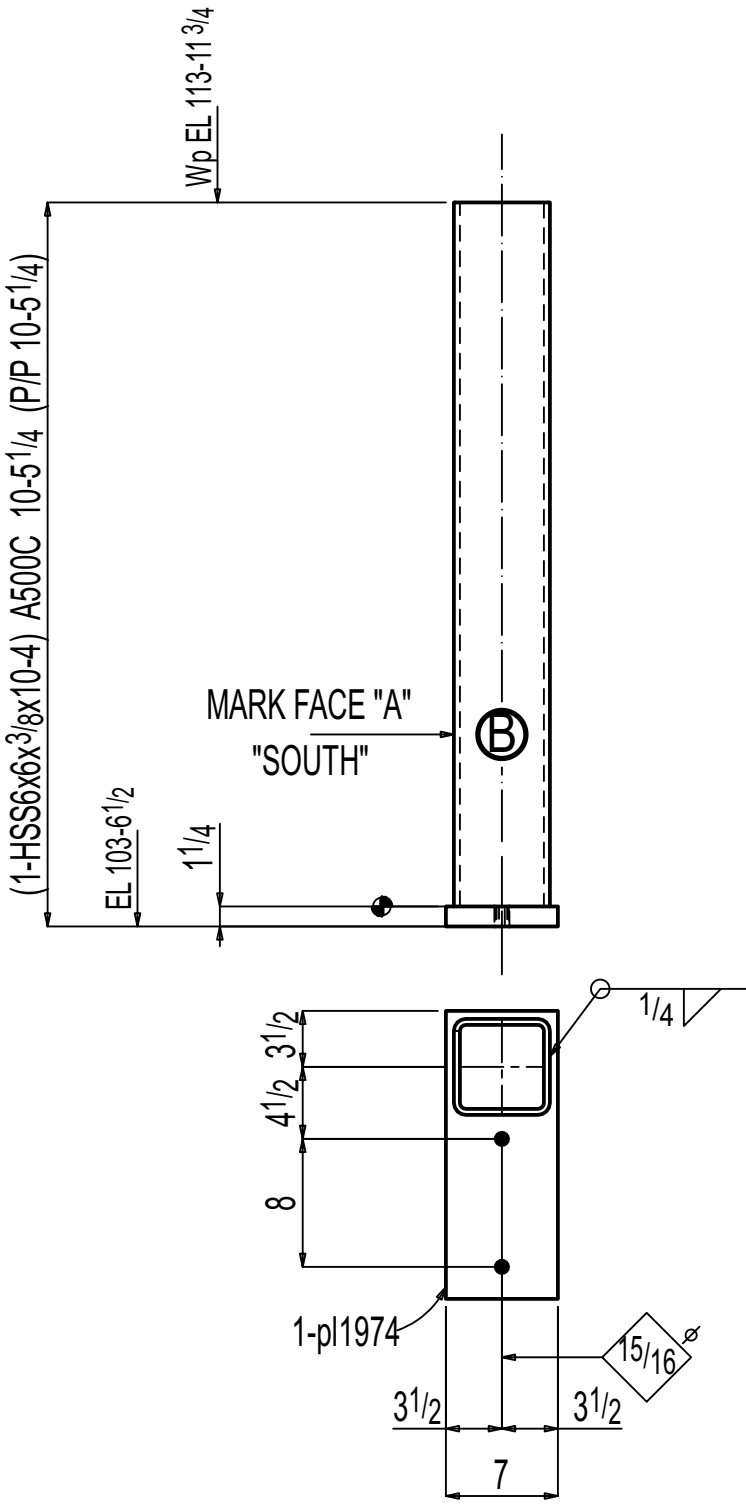
ONE COLUMN F-12.02C1
