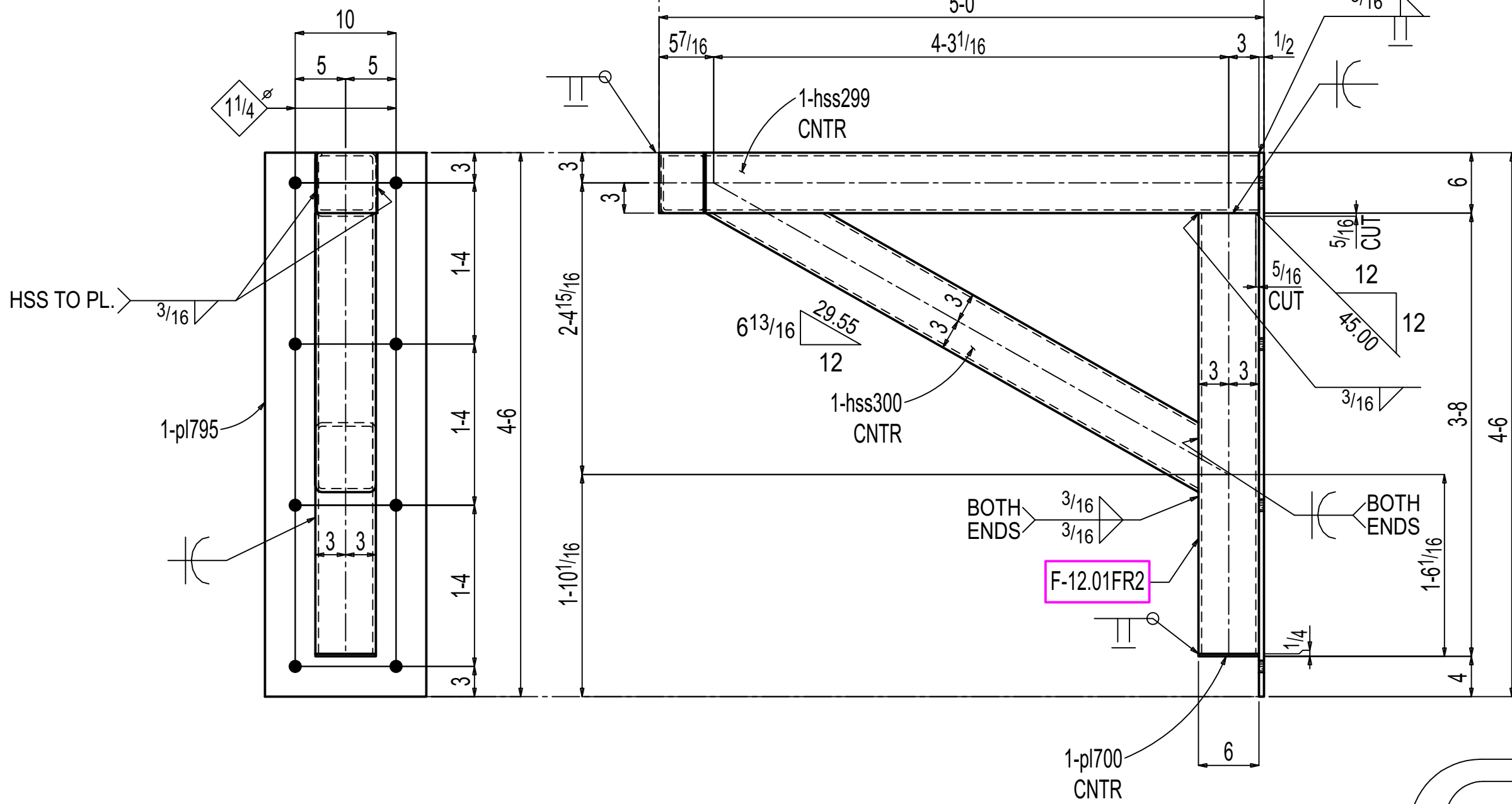
ONE FRAME F-12.01FR2
