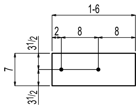
ONE LEVELING PLATE F-12.01LP1
