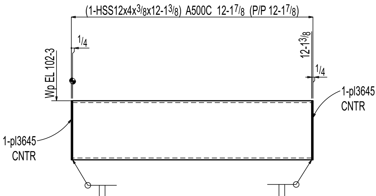
ONE BEAM F-12.02B2
