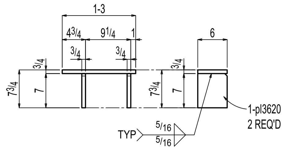
ONE PLATE F-12.01M2
