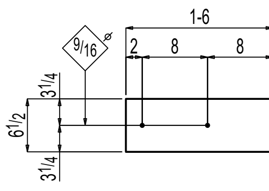
ONE LEVELING PLATE F-12.01LP2
